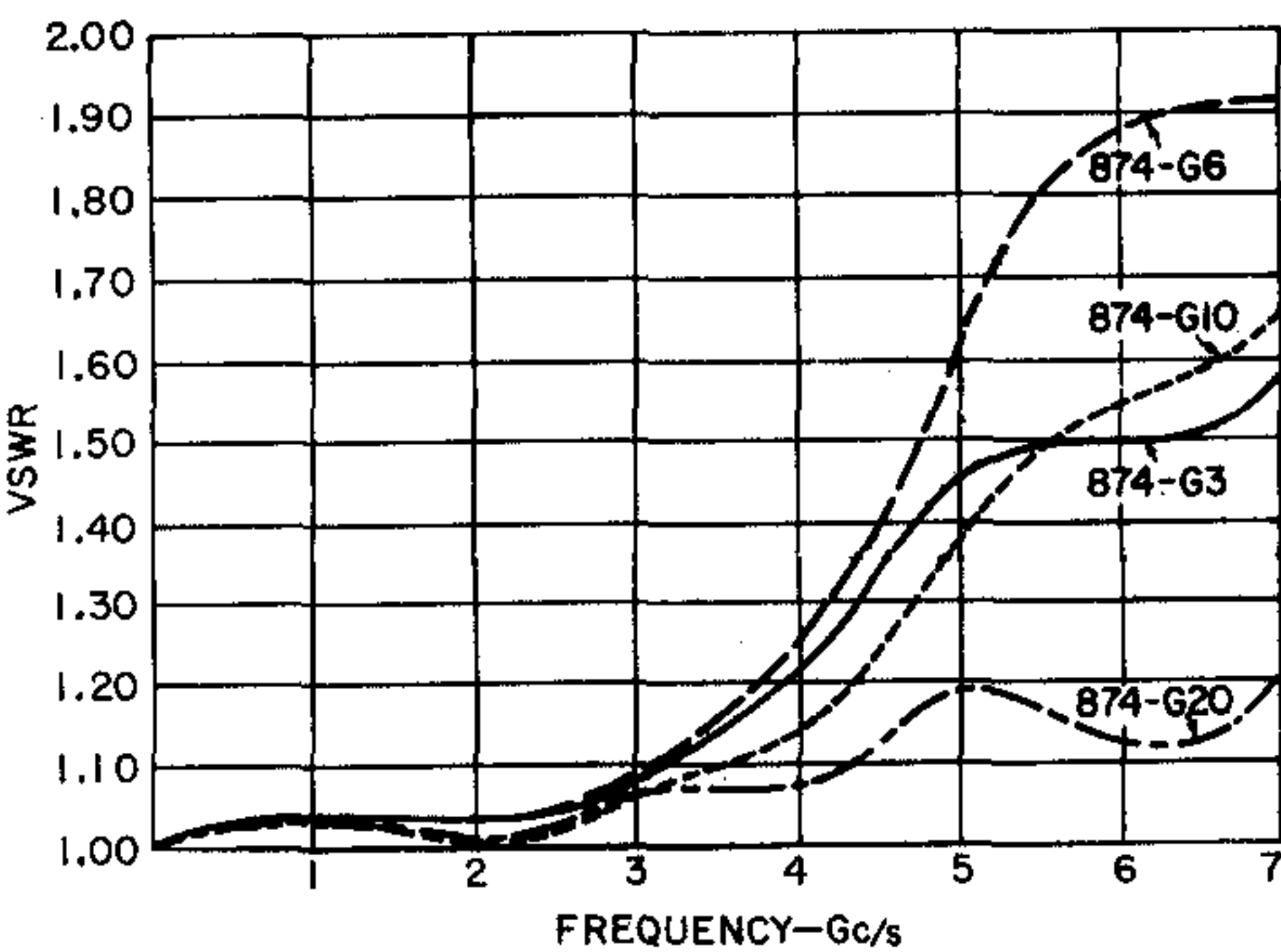
Figure 1. Typical VSWR of Type 874-G Attenuators.
